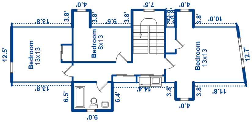
Third Floor 786.8 sf
